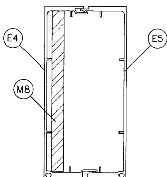
MULLION 'M4A'
