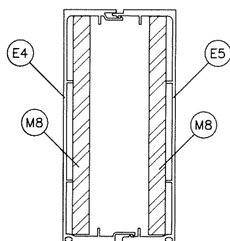
MULLION 'M4'
