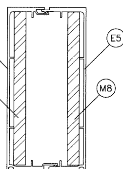
MULLION 'M4'
