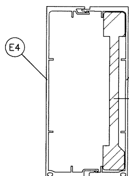
MULLION 'M2'
