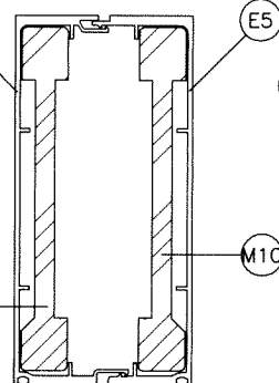
MULLION 'M3'
