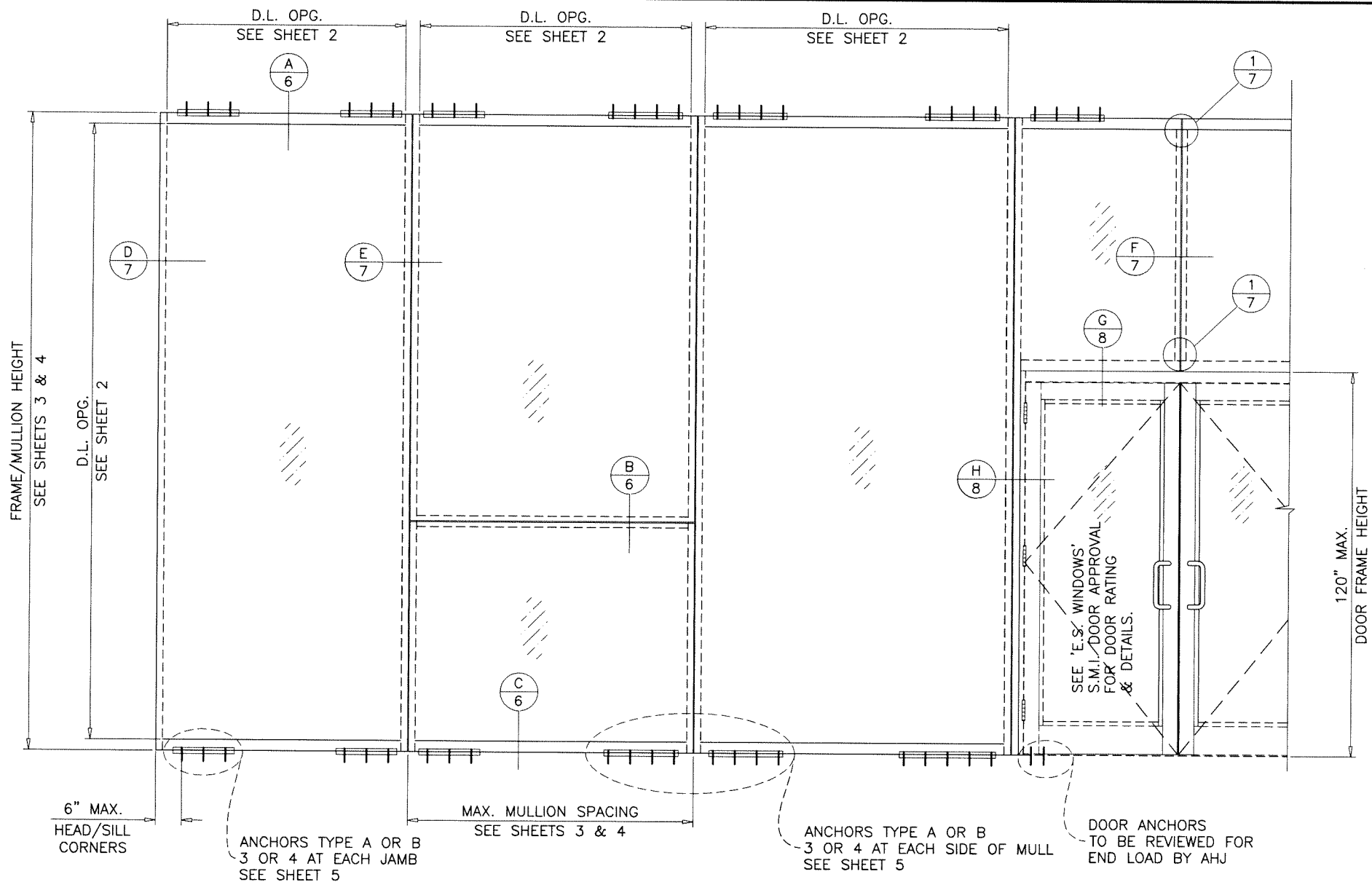
TYPICAL ELEVATIONS
